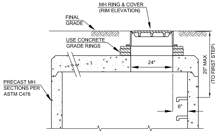
FLAT-TOP SECTION
